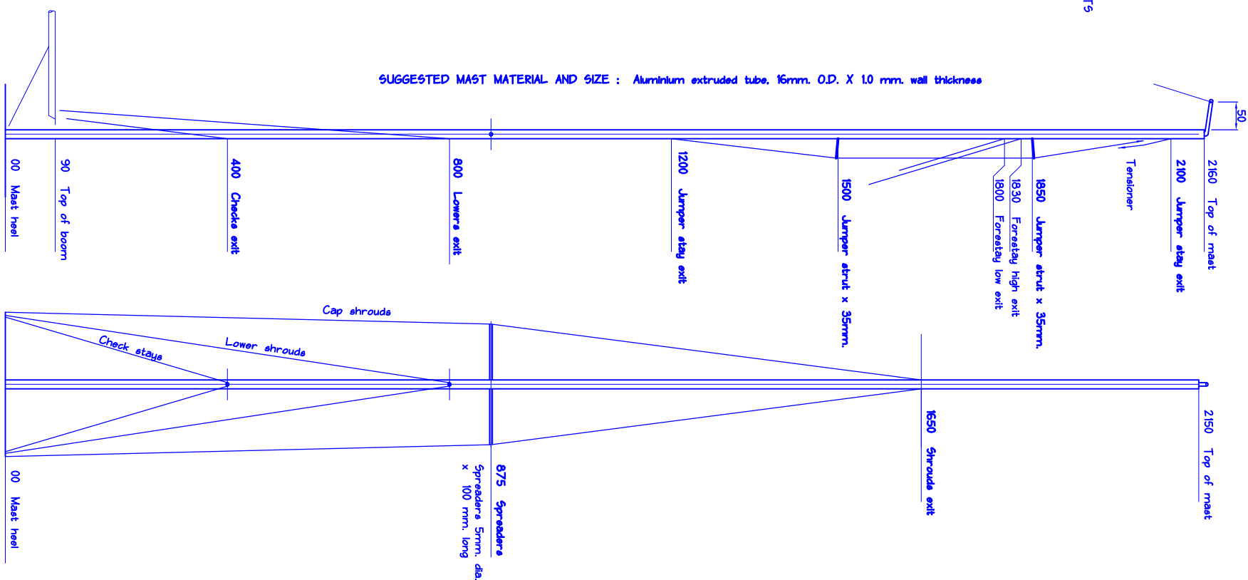
MAST STANDING RIGGING
