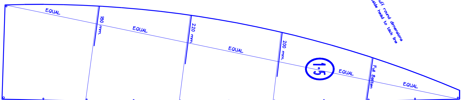
MAIN GULL PANEL LAYOUT (0.65m 2 )
