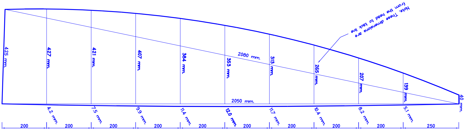
MAIN GULL DIMENSIONS (0.65m 2 )
