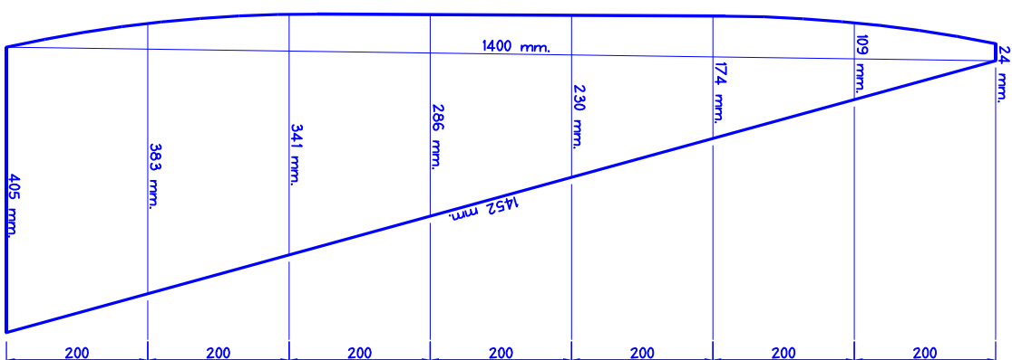
JIB DIMENSIONS (0.35m 2 )
