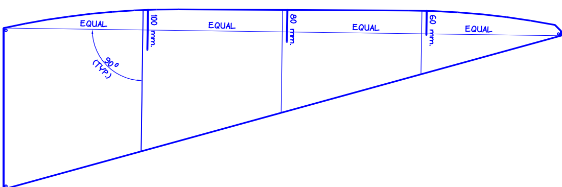
JIB PANEL LAYOUT (0.35m 2 )
